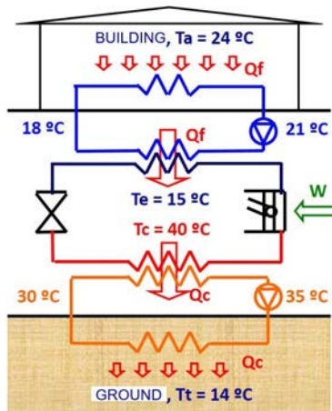
Active cooling
