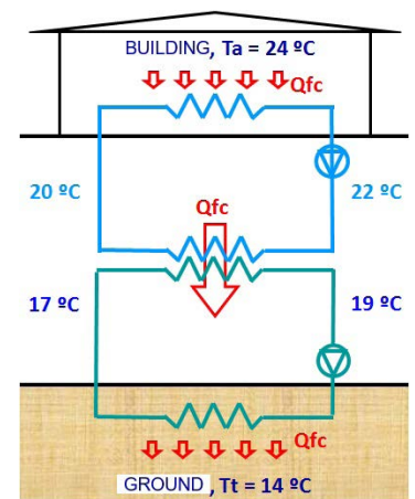
Passive cooling
