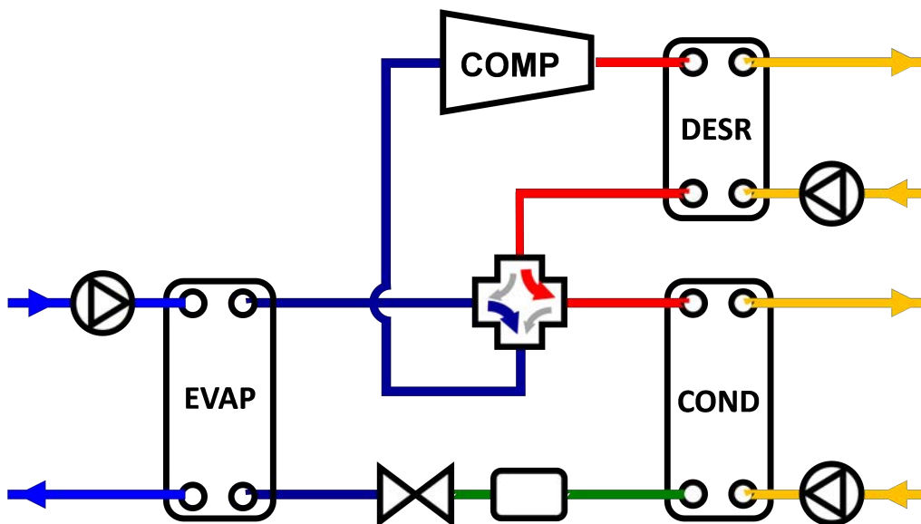
Simplified scheme of a CLASSIC HC with desuperheater.
