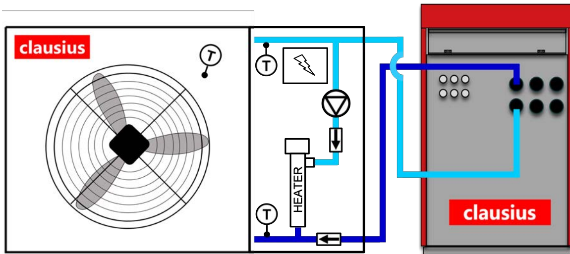
Simplified diagram, CLAUSIUS air System
