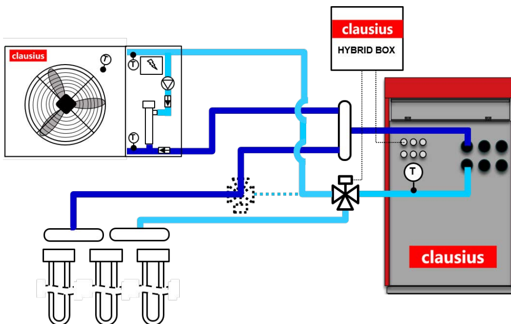
Simplified scheme, CLAUSIUS Hybrid System
