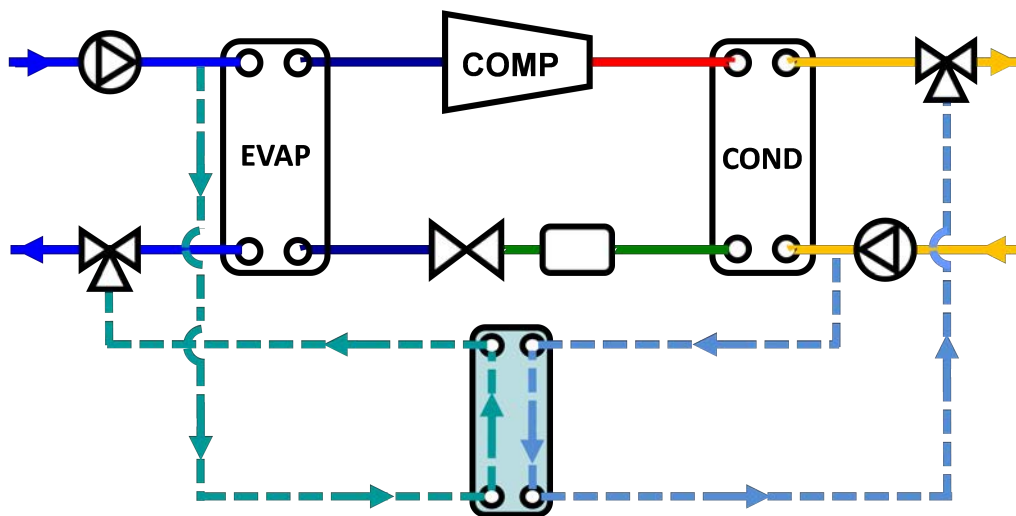
Simplified scheme of the passive cooling production system.
