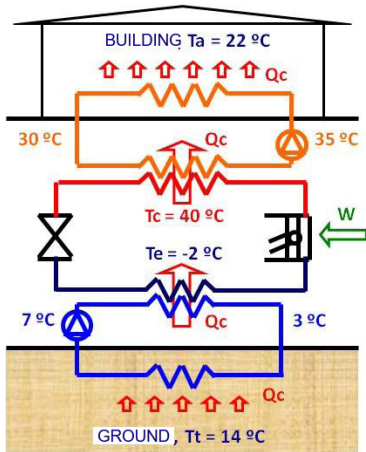
Heating
