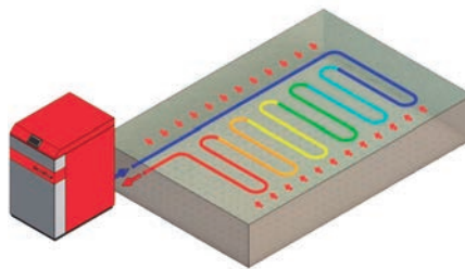
Horizontal ground collector
